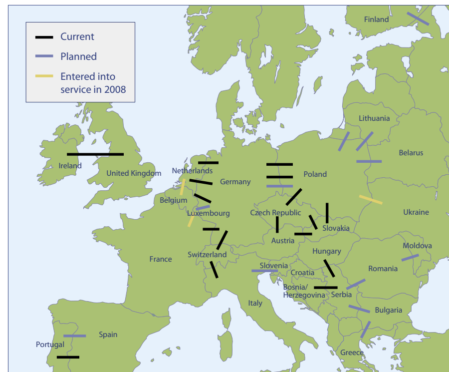
Map 3.8.2 – Cross-border dark fibre
