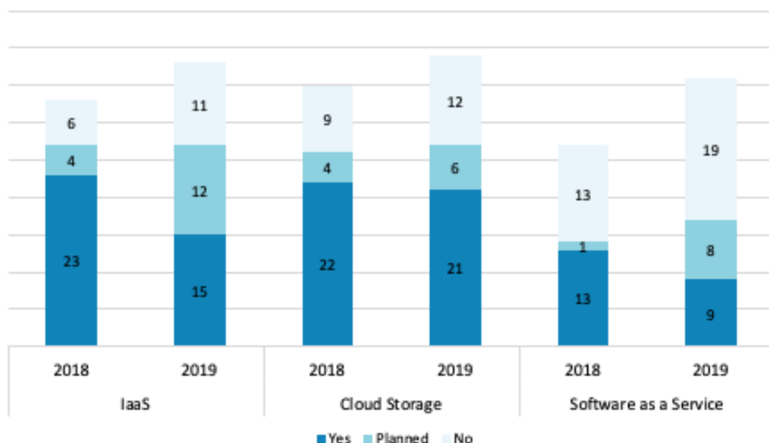
Figure 8.1: Availability of cloud services from NRENs
