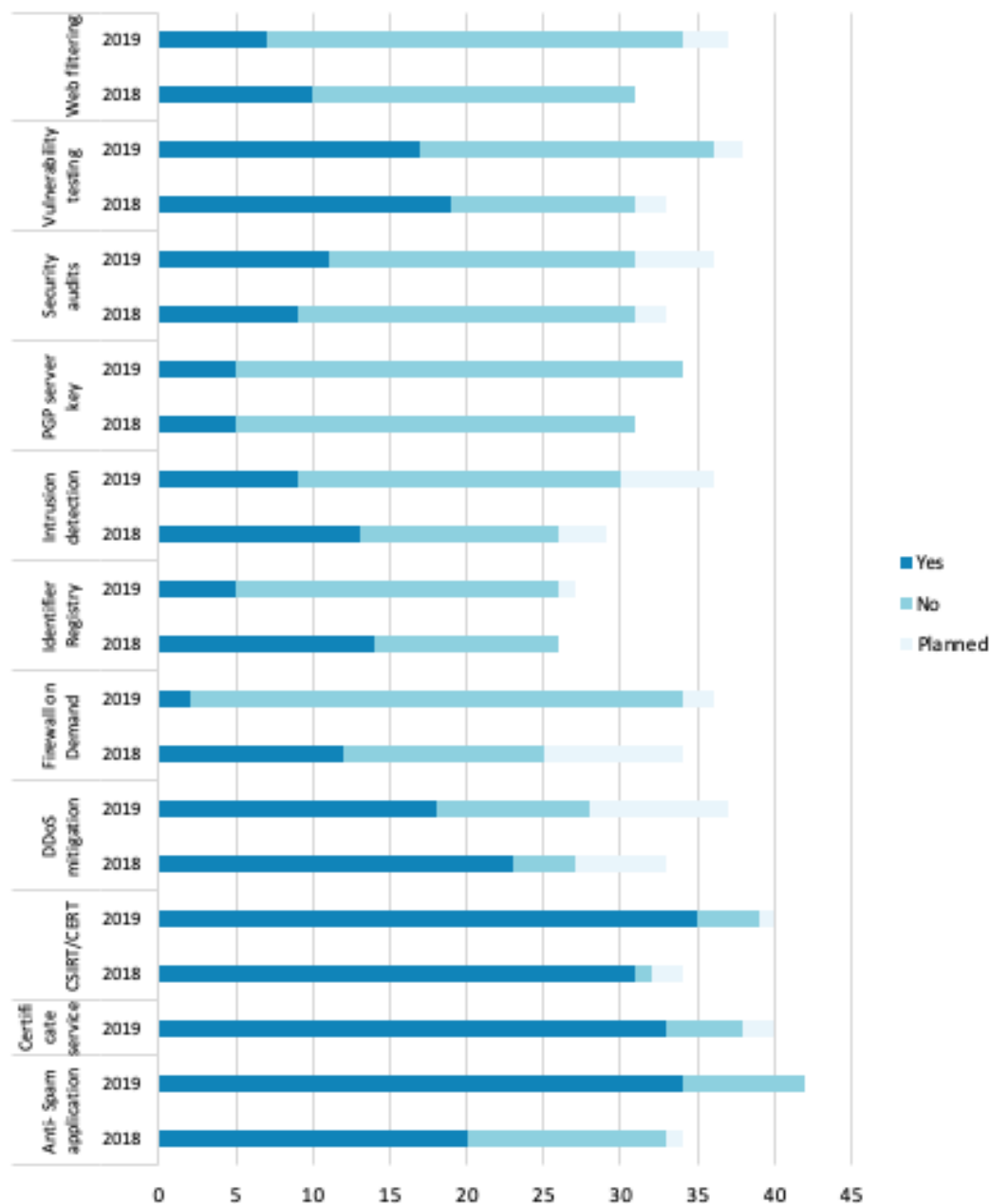
Figure 6.2: Security services offered by NRENs.
