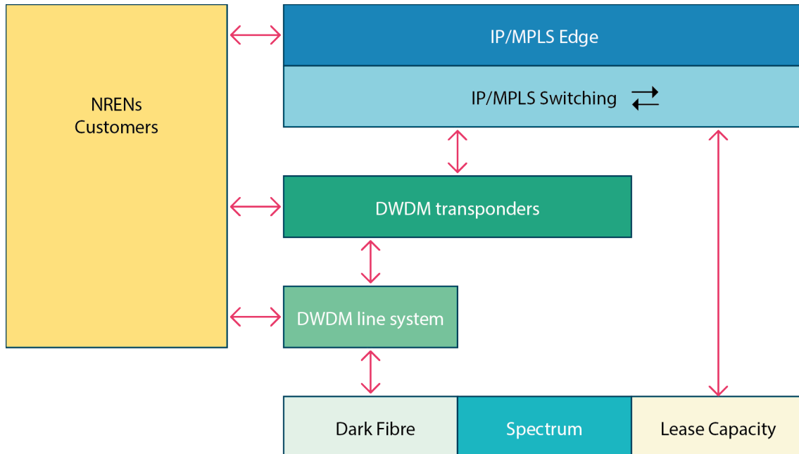
Figure 5.14: Layers of the network as it will be after the transition to a partly disaggregated DWDM system The three layers are transport, transmission (in green) and packet (in blue). The transmission portion of the network will be composed of only two blocks (OTN switching having been removed), which will be independent of each other. NRENs (and other customers) will be able to connect to either block to access existing point-to-point high-capacity Ethernet services (today, Lambdas) as well as the new upcoming Spectrum Connection Service (when connecting directly to the DWDM line system).
