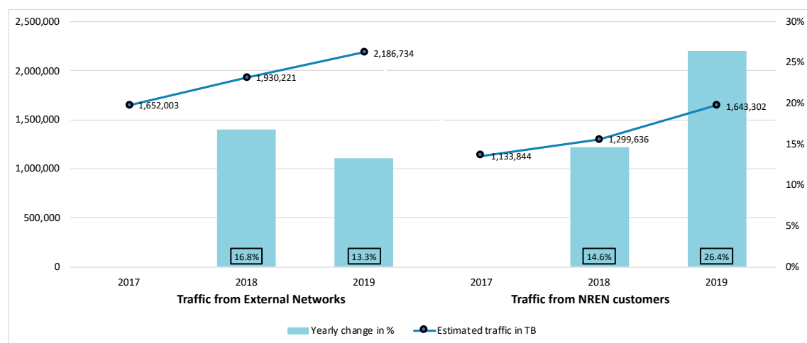
Figure 5.1: Increase of traffic into the NRENs from external networks (left-hand graph) and NREN end users (right-hand graph) 2017 to 2019
