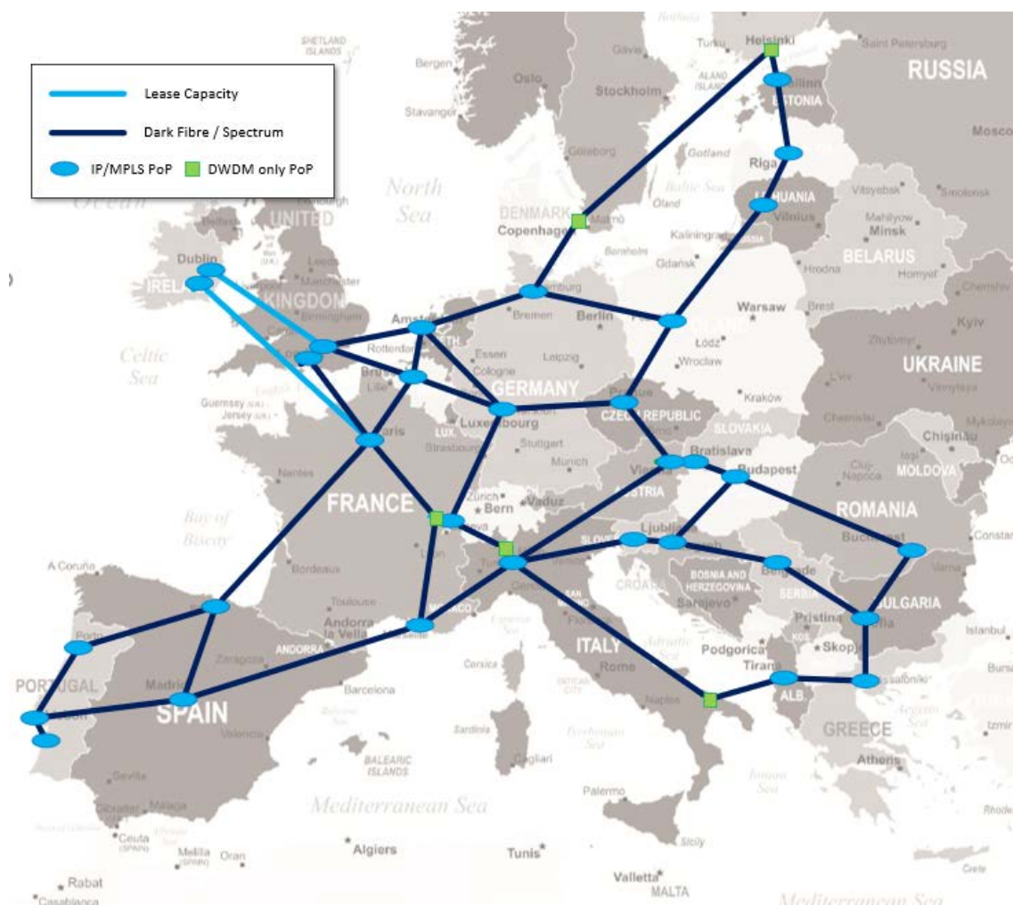
Figure 5.13: A view of the current reference topology for GN4-3N
